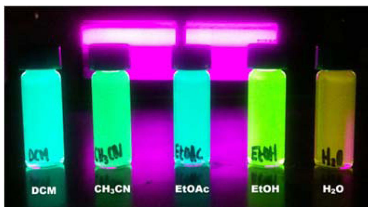
Figure 3. Compound 5a in five different solvents (ranging from relatively nonpolar DCM to highly polar H 2 O) under long wavelength UV light (365 nm) displaying intense solvatochromism (photo taken with 3 megapixel camera; color unaltered).
