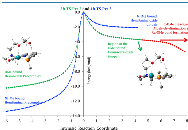
Figure 9. Intrinsic reaction coordinates originating from 3b -TS-Prt-2 (hemiacetal; green curve) and 4b -TS-Prt-2 (hemiaminal; blue curve). M06 gas phase electronic energies defined relative to the TSs in kcal/mol.
