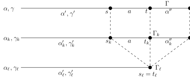
Fig. 4. Proof of Theorem 7: illustration of case one.
