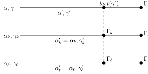
Fig. 5. Proof of Theorem 7: illustration of subcase 2.1.
