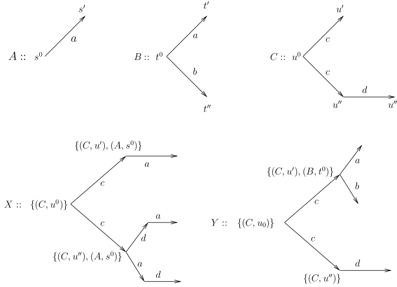
Fig. 7. The Automata in Example 1.
