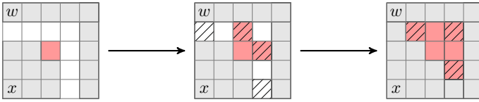
Fig. 2. In Lemma 5.9, a modification of x in the boundary of F_n only affects the value of z(x, n) in a bounded region
