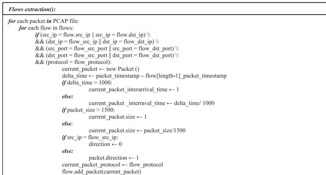
FIGURE 4 Flow extraction algorithm. PCAP, packet capture
